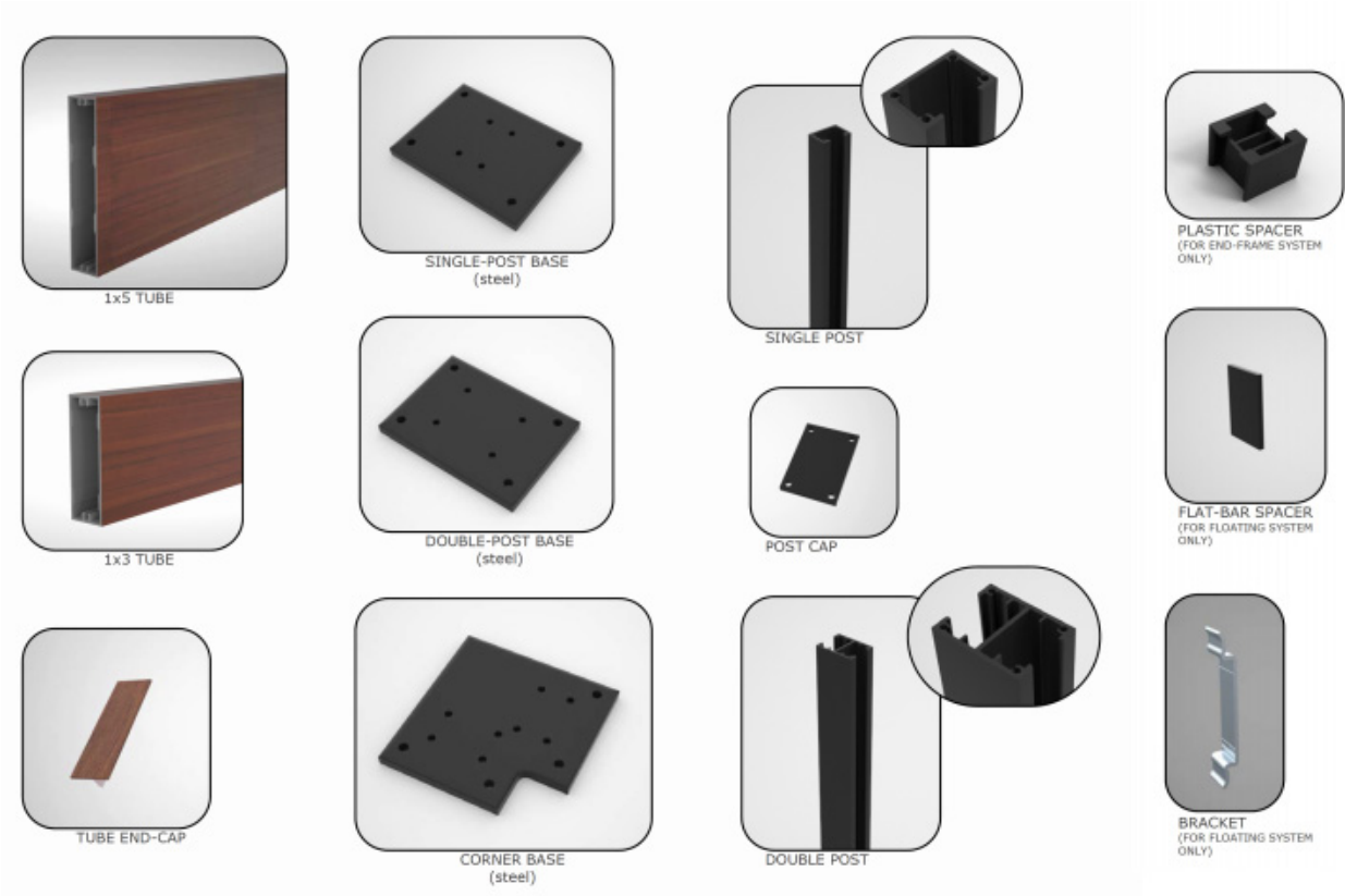
FIGURE 2—LONGBOARD PRIVACY SCREEN SYSTEM COMPONENTS
