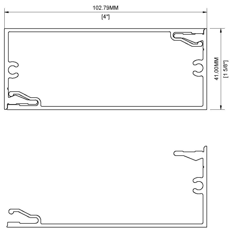
FIGURE 3—LINK & LOCK BATTENS (4-INCH PIECE TUBE AS SHOWN, ALSO AVAILABLE IN 6 AND 8-INCH TUBES)
